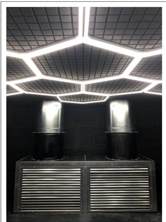
Ezi-Duct modular ducting system installed at the men's shed.
